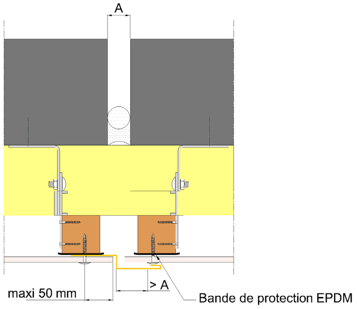
Figure 18 - Joint de dilatation
