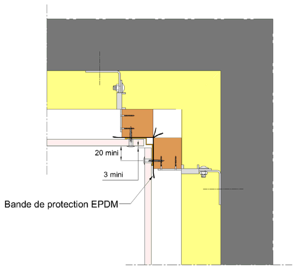
Figure 13 – Angle rentrant
