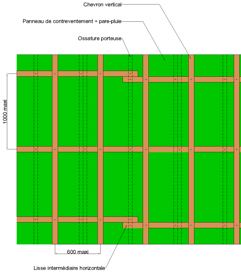
Figure 21 - Raccordement de lisses horizontales - Pose sur COB
