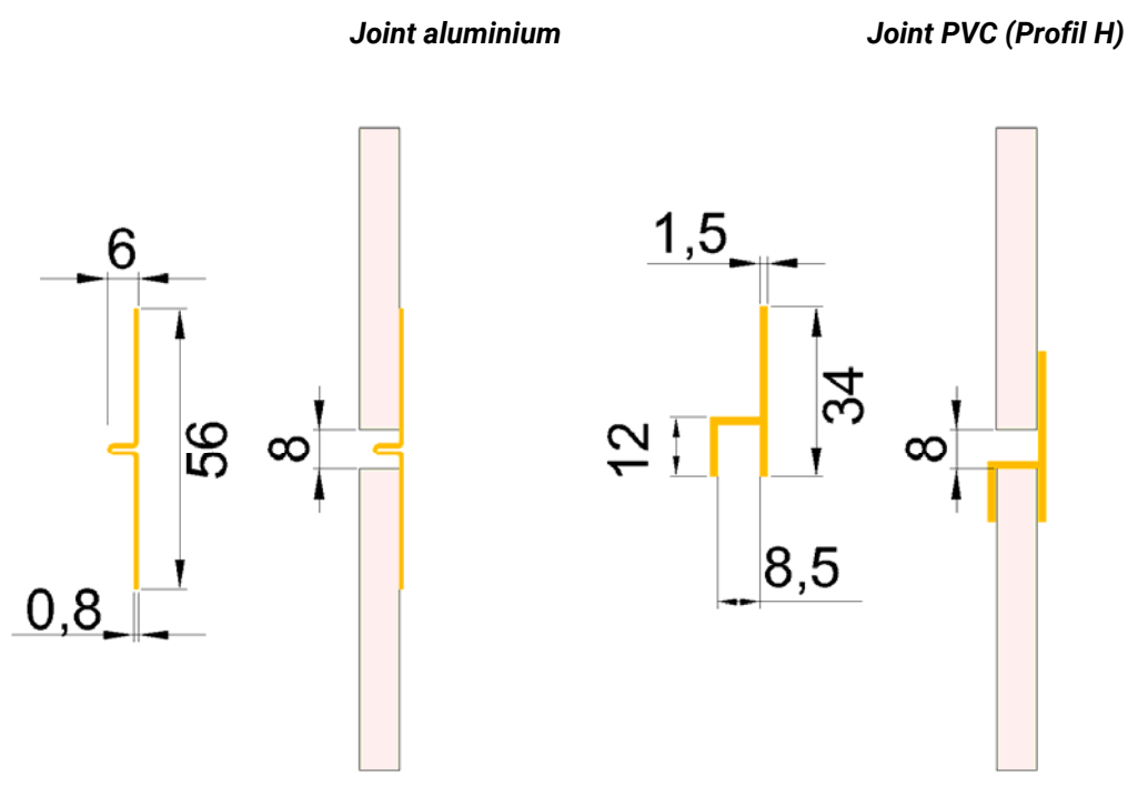
Figure 7 - Types de profilés de joint horizontal
