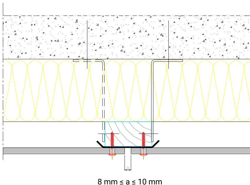
Figure 13 – Joint vertical
