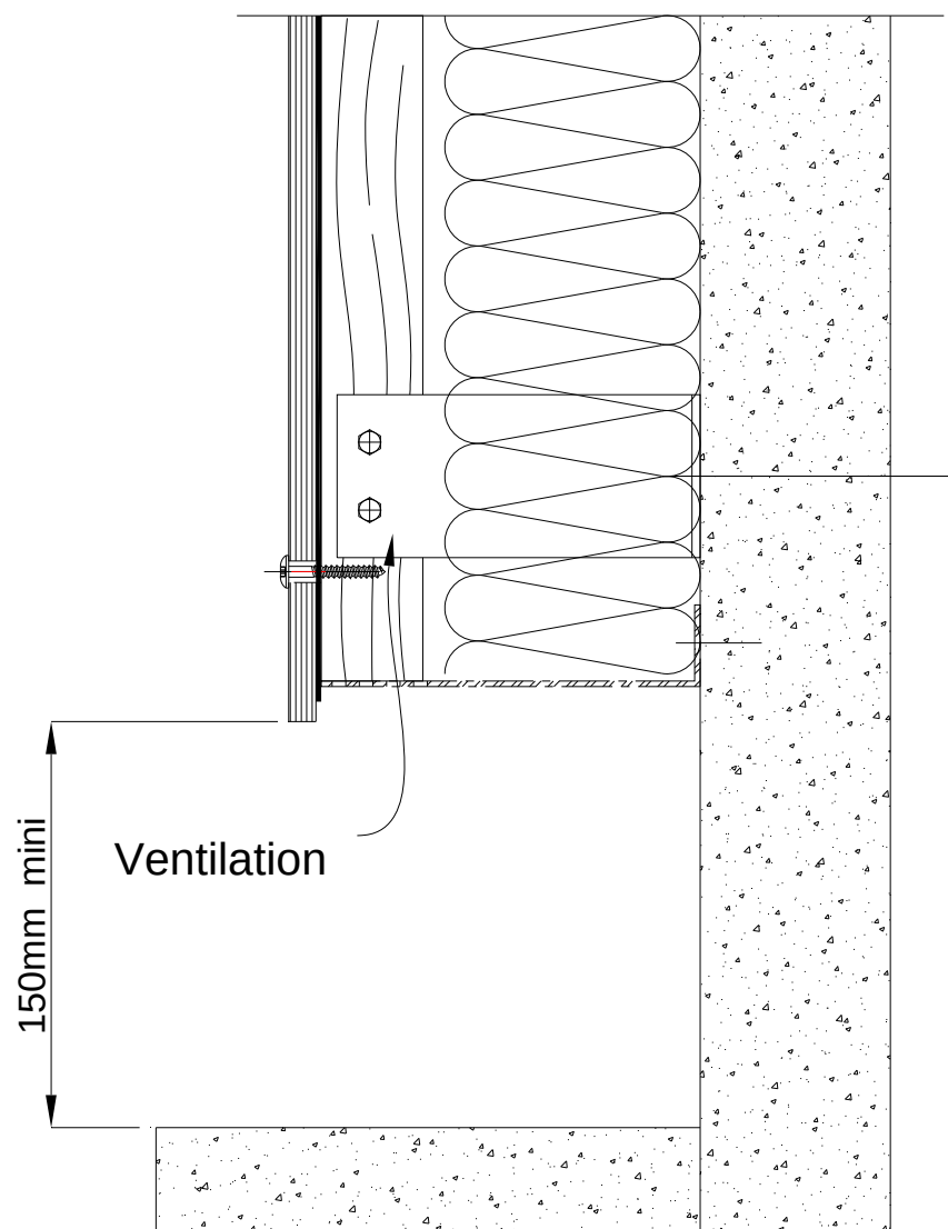
Figure 5 – Départ
