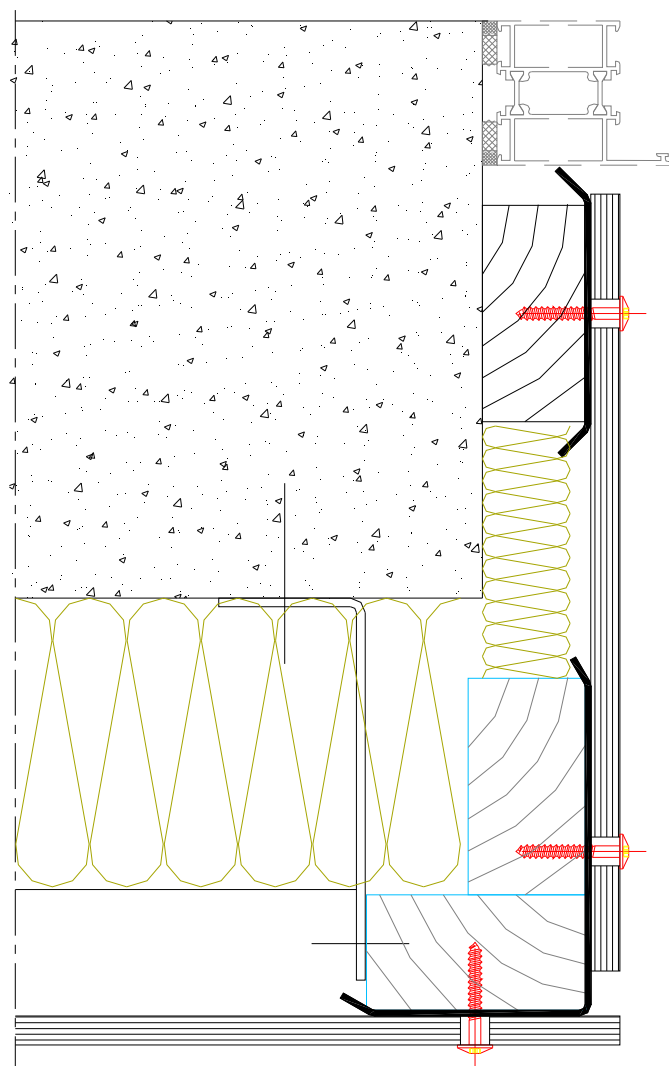
Figure 8 – Retour tableau
