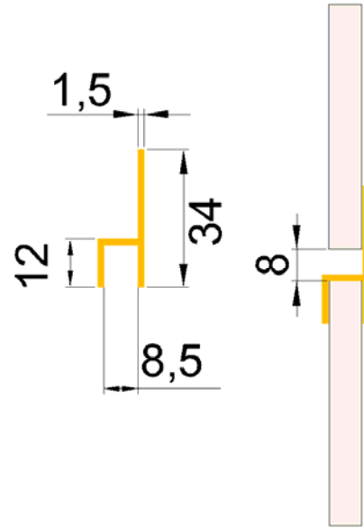
Joint PVC (Profil H)
