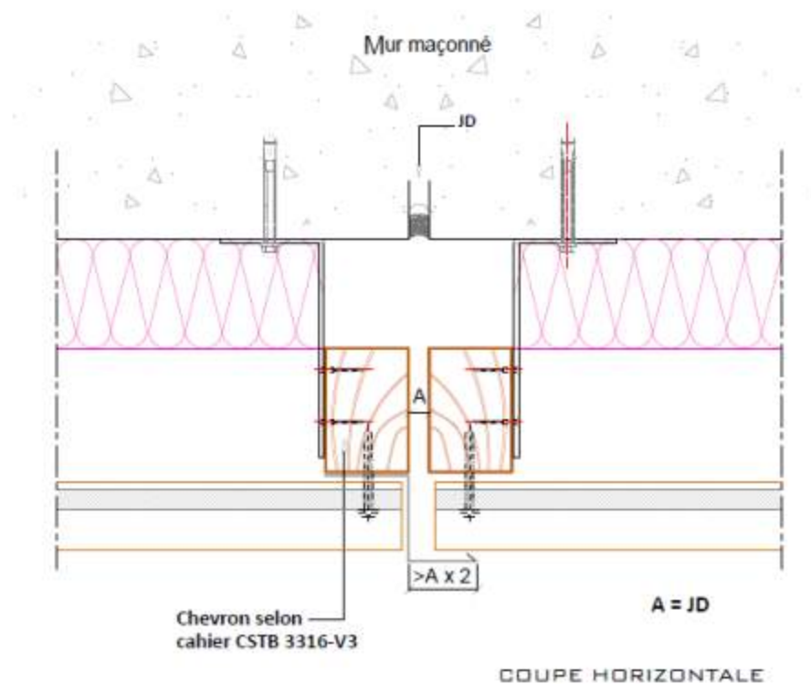
Figure 12 – Joint dilatation
